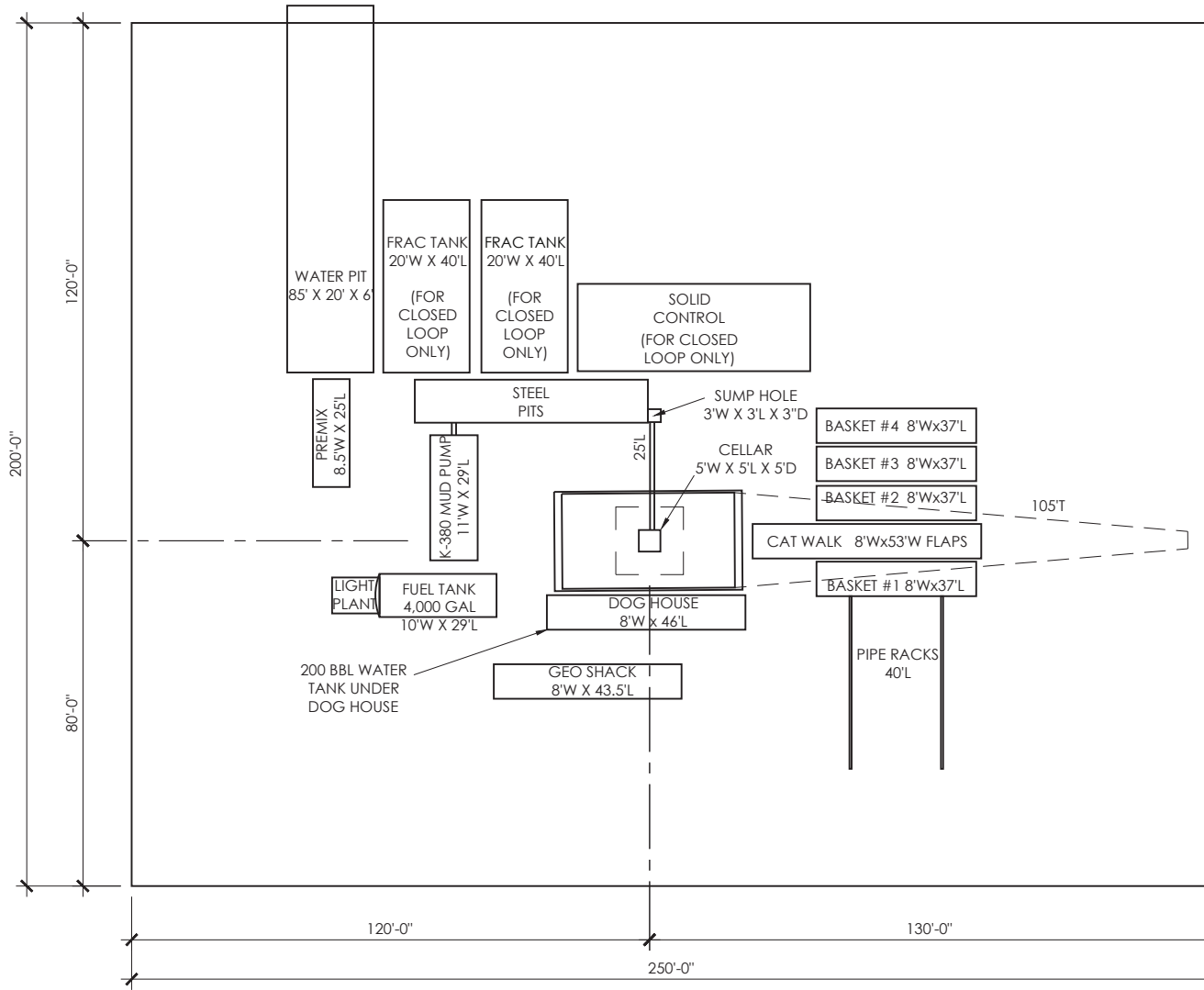
250' x 200' Rig #112 Steel Pit Setup KB 8'
