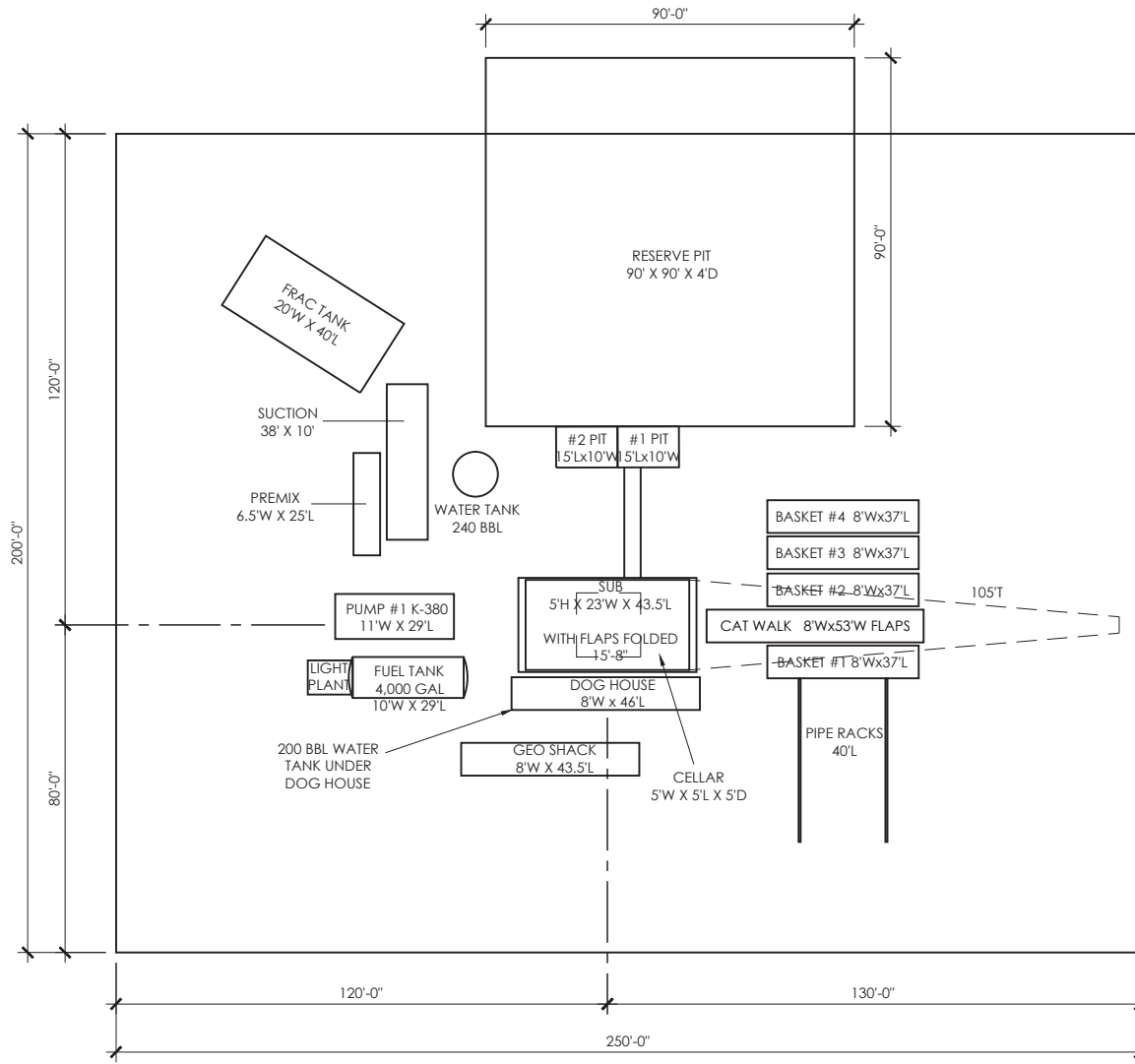
250' x 200' Rig #112 with Earth Pits KB 8'
