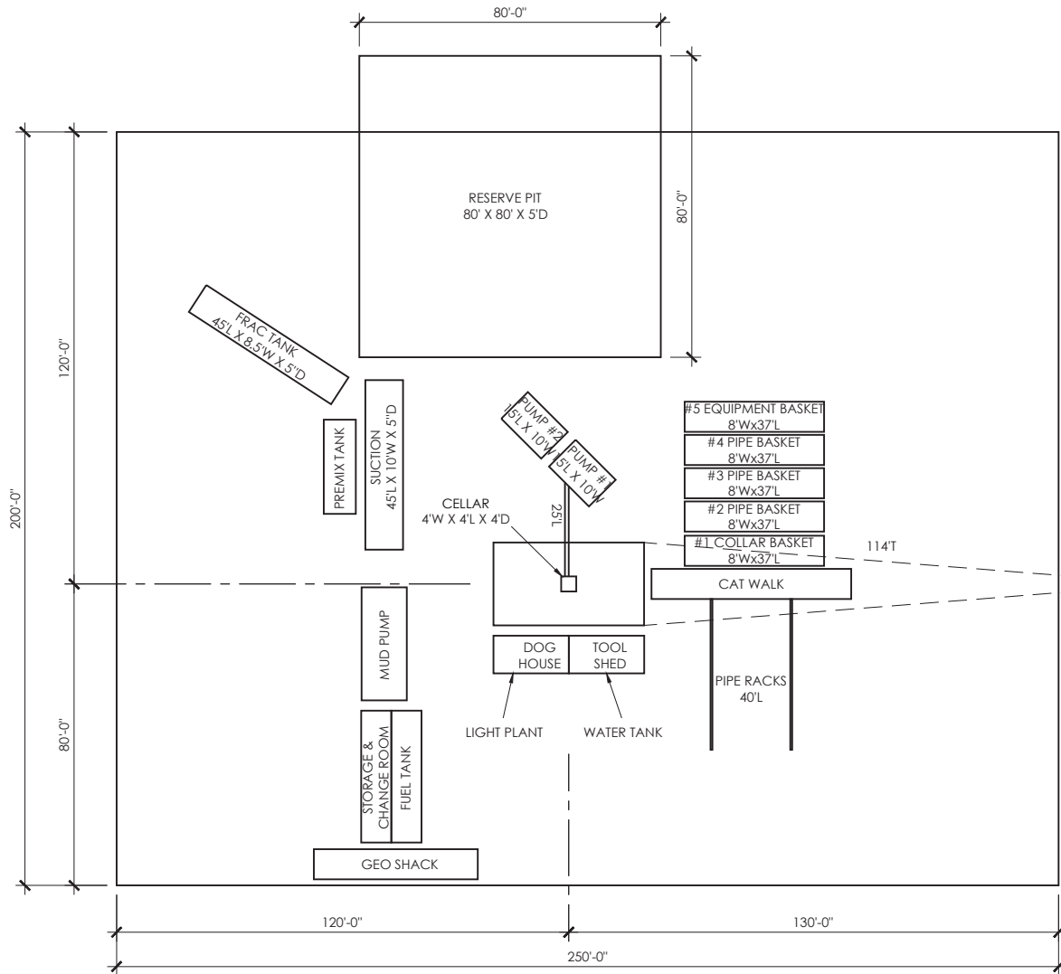
250' x 200' Rig #114 with Earth Pits KB 8'
